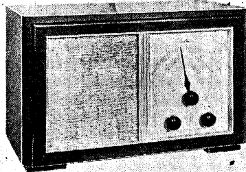
The appearance of the Beethoven A415 A.C. superhet. The complete front, including speaker and scale as seen here, is withdrawn forward to dismantle the set.
